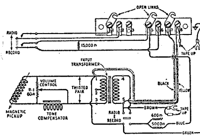
Figure 10—Connections for Attaching Portable Turntable Model PT-23
